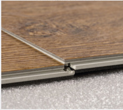
FIG. 5 Using the 3L TripleLock one piece drop-lock system, drop the short side of plank (3) onto the short side of plank (1). Be sure to align the short side of the row so it is not too tight or too loose.
