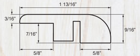
55 LFSTN FLUSH STAIR NOSE
